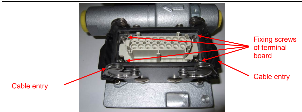
Figure 22: Socket housing
