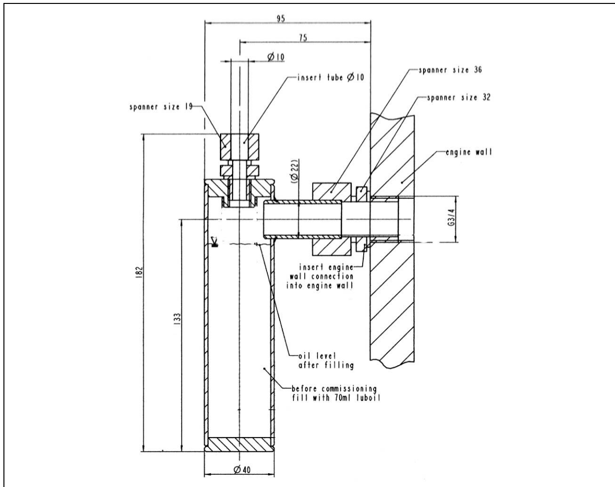
Figure 12: Pipe siphon
