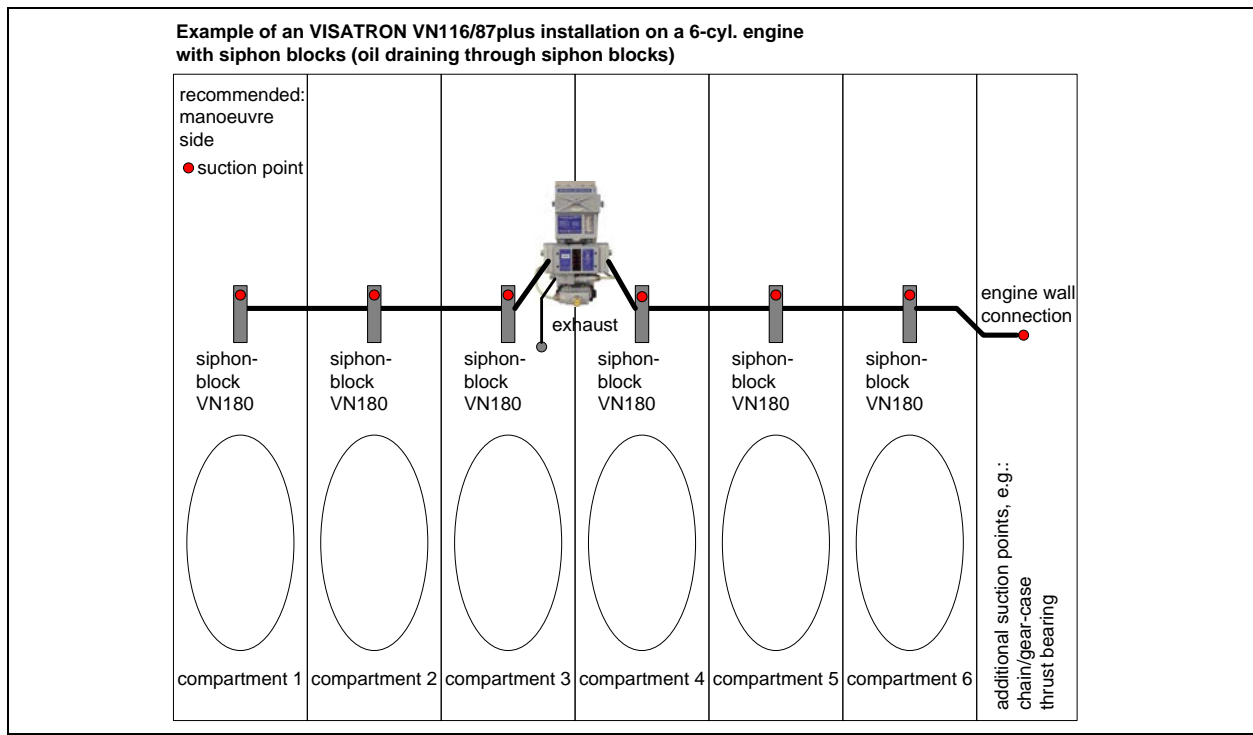
Figure 9: Alternative installation of VN116/87plus OMD
