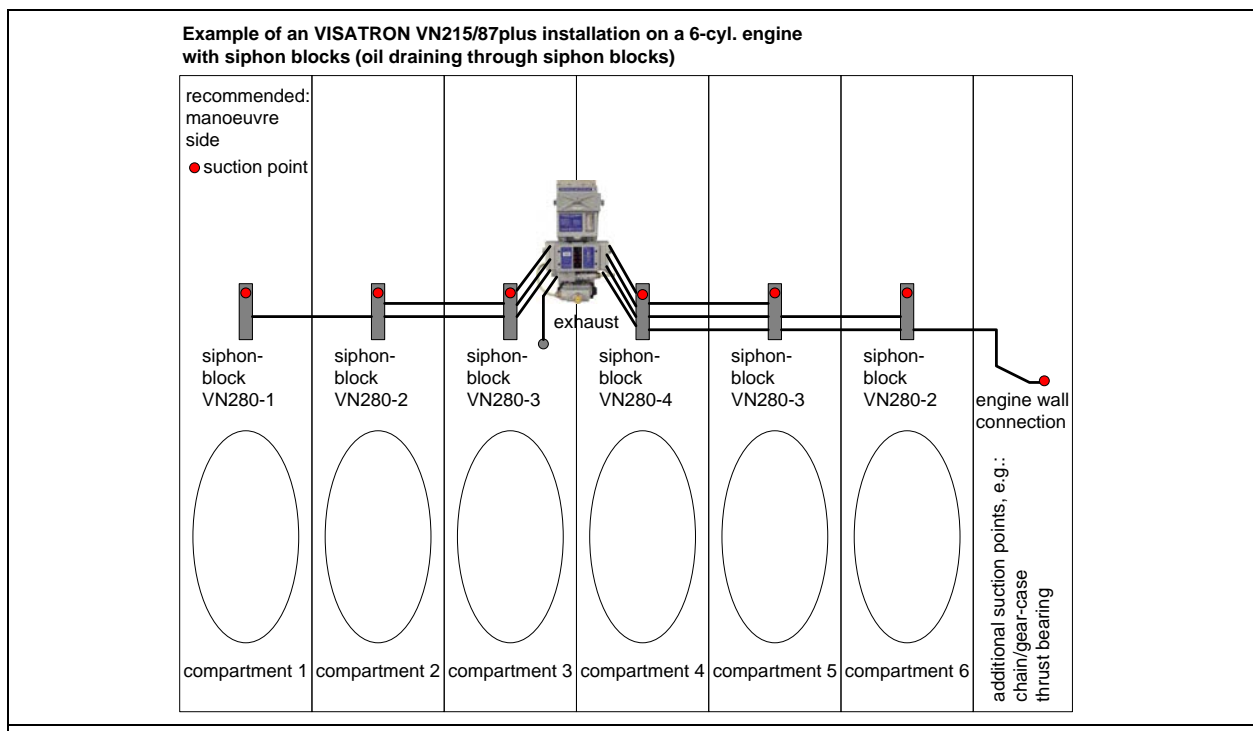
Figure 10: Recommendation for best VN215/87plus OMD installation
