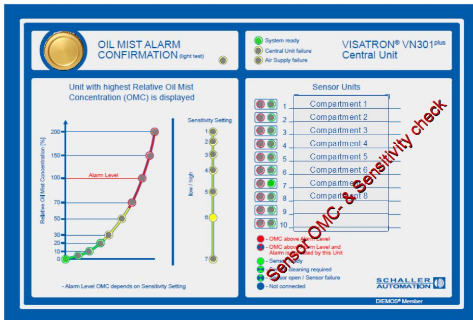
Figure 21: Display of the VISATRON® VN301 plus / VN301 plus EX System performing a Sensor OMC- and sensitivity check. The next sensor is displayed by pushing the Oil Mist Alarm Confirmation button within 20 seconds.
