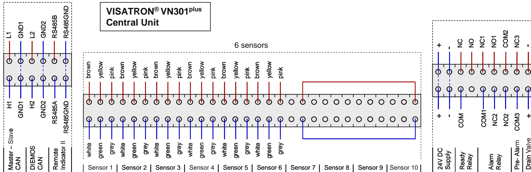
Figure 11: VISATRON® VN301 plus / VN301 plus EX Central Unit electrical wiring for six sensors.
