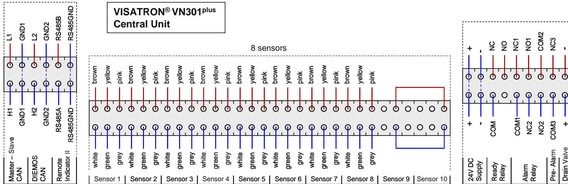
Figure 13: VISATRON® VN301 plus / VN301 plus EX Central Unit electrical wiring for eight sensors.
