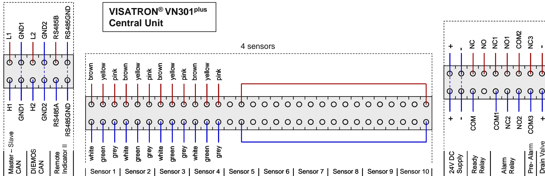
Figure 9: VISATRON® VN301 plus / VN301 plus EX Central Unit electrical wiring for four sensors.
