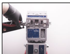
2. Using circlip pliers, change the scavenging air filter.
