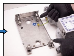
15. Check the upper and lower suspensions for any damage, replace if necessary.
